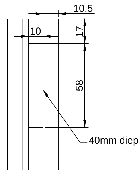
Detail D
