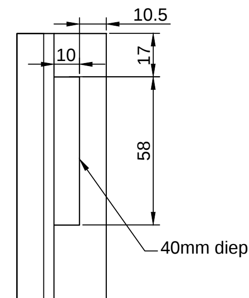
Detail D
