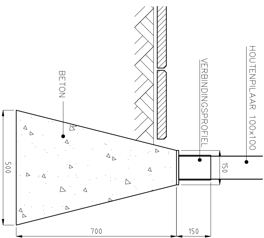
PRINCIPE DETAIL FUNDERING Schaal 1:10
