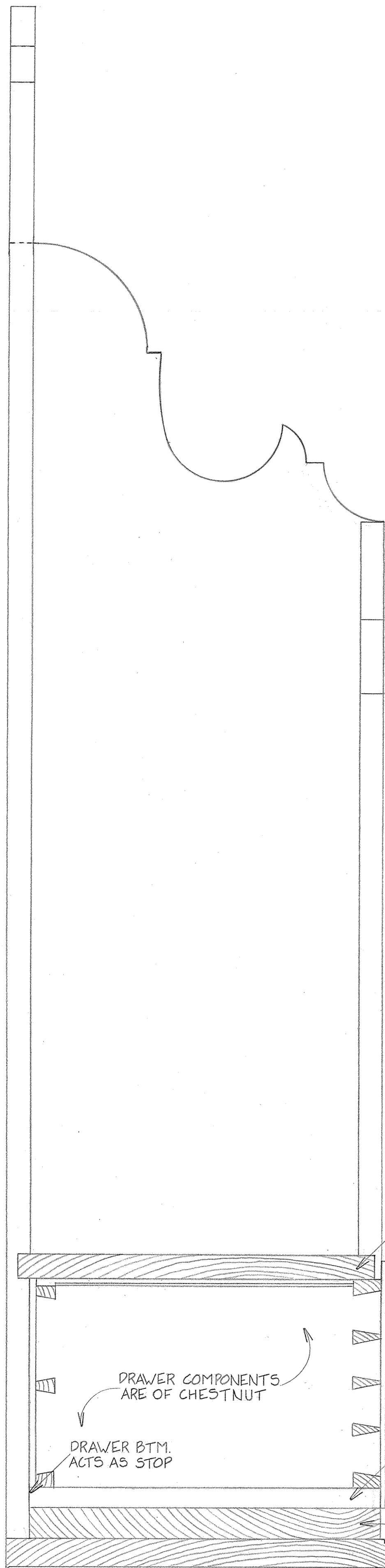
SECTION THRU SIDE FULL SIZE
