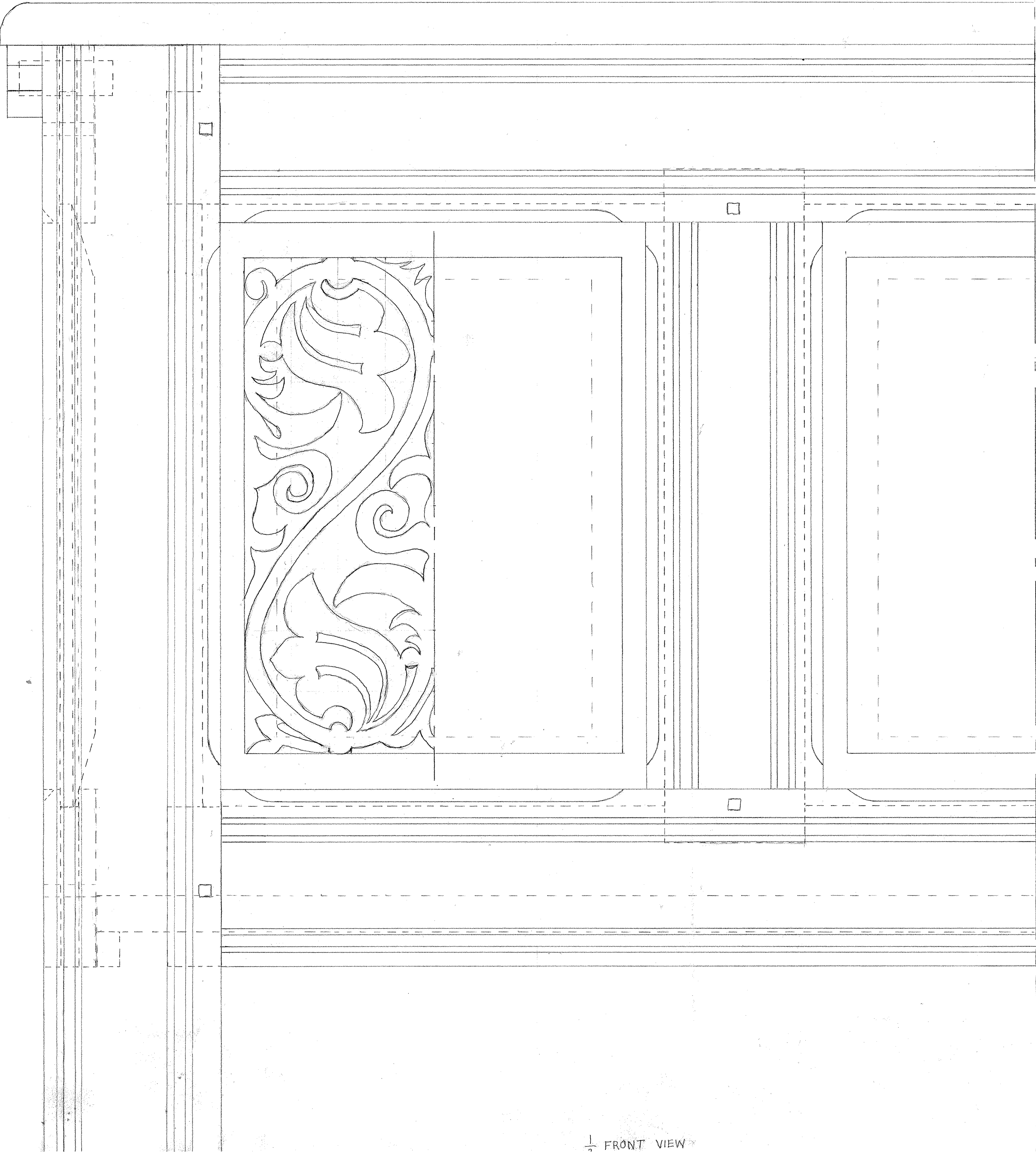
1/2 FRONT VIEW
