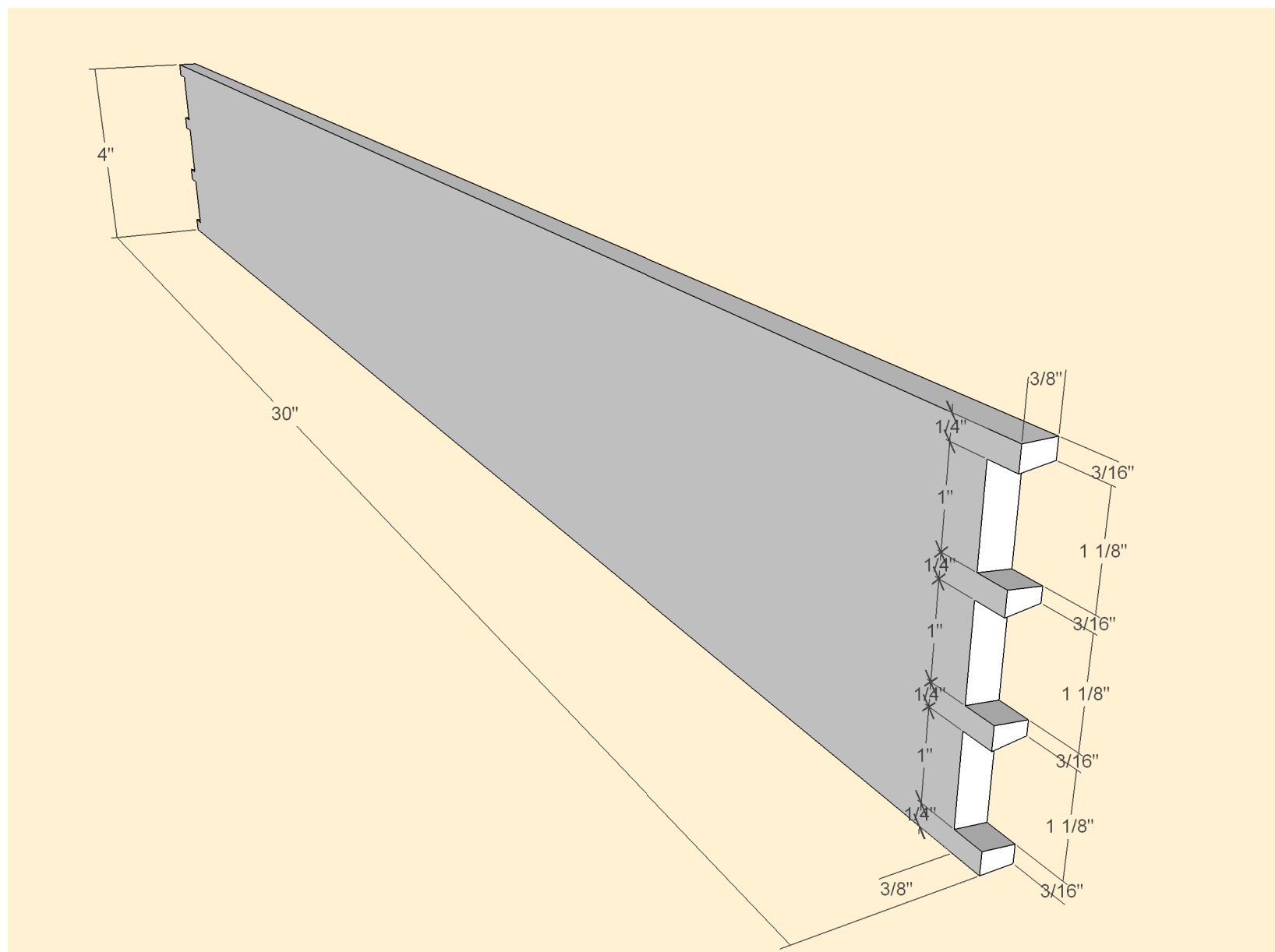
Drawer Back and Dovetail Joint
