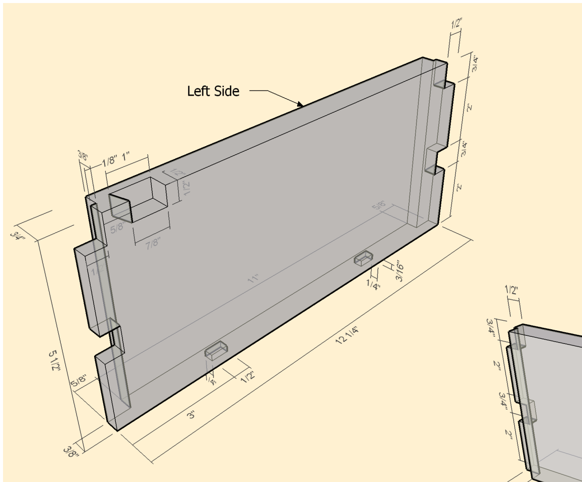
Left Side Inside View
