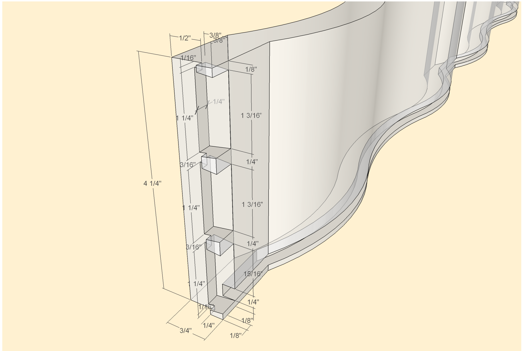
Drawer Front Dovetail Joint
