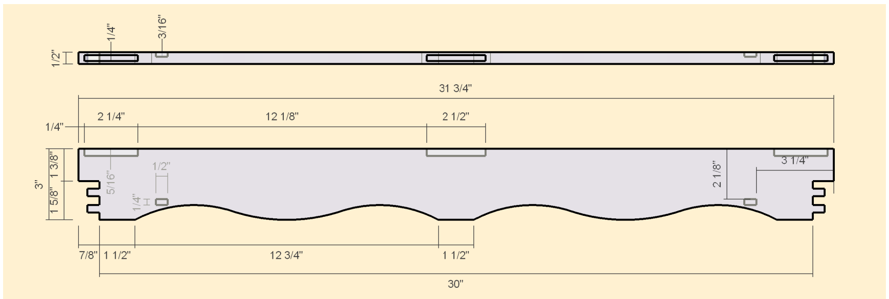
Bottom Rail Top View
