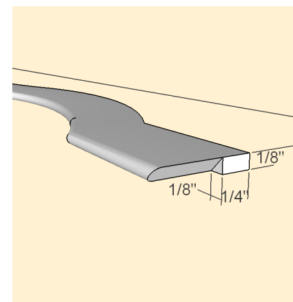
Top Cock Bead Joint
