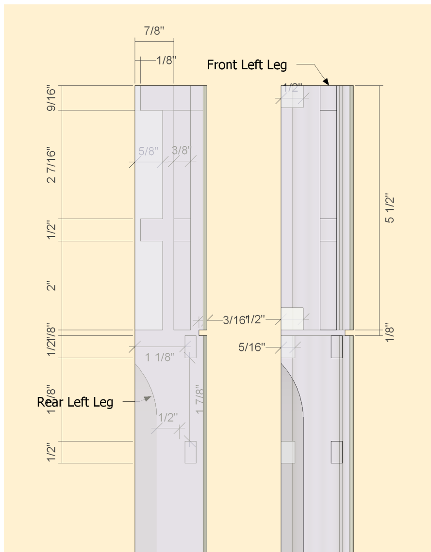
Legs Back View Orthographic
