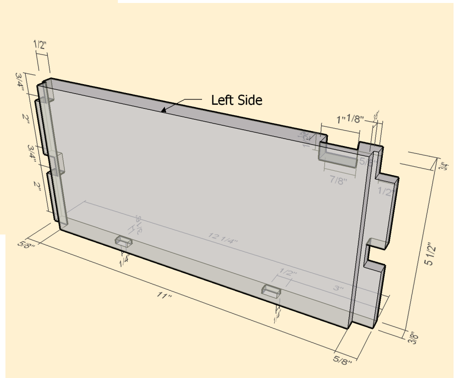
Left Side Outside View
