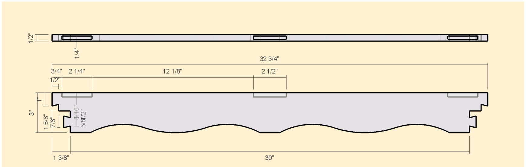
Top Rail Top View
