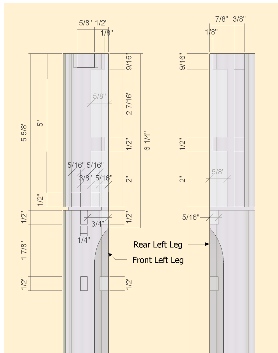
Legs Right View Orthographic
