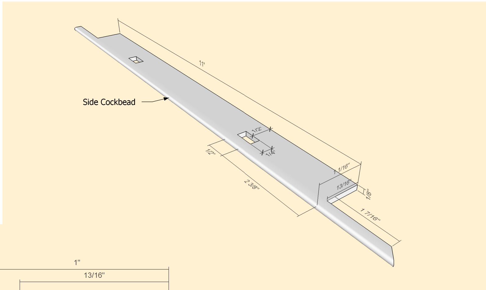
Side Cock Bead
