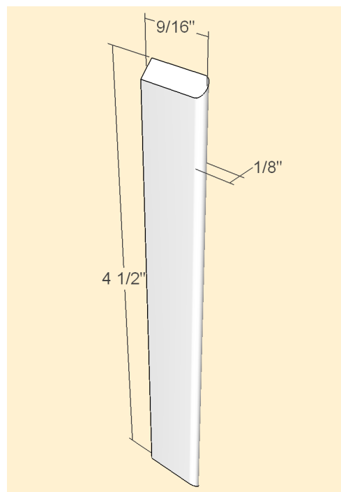
Drawer Cock Bead - Top and Bottom
