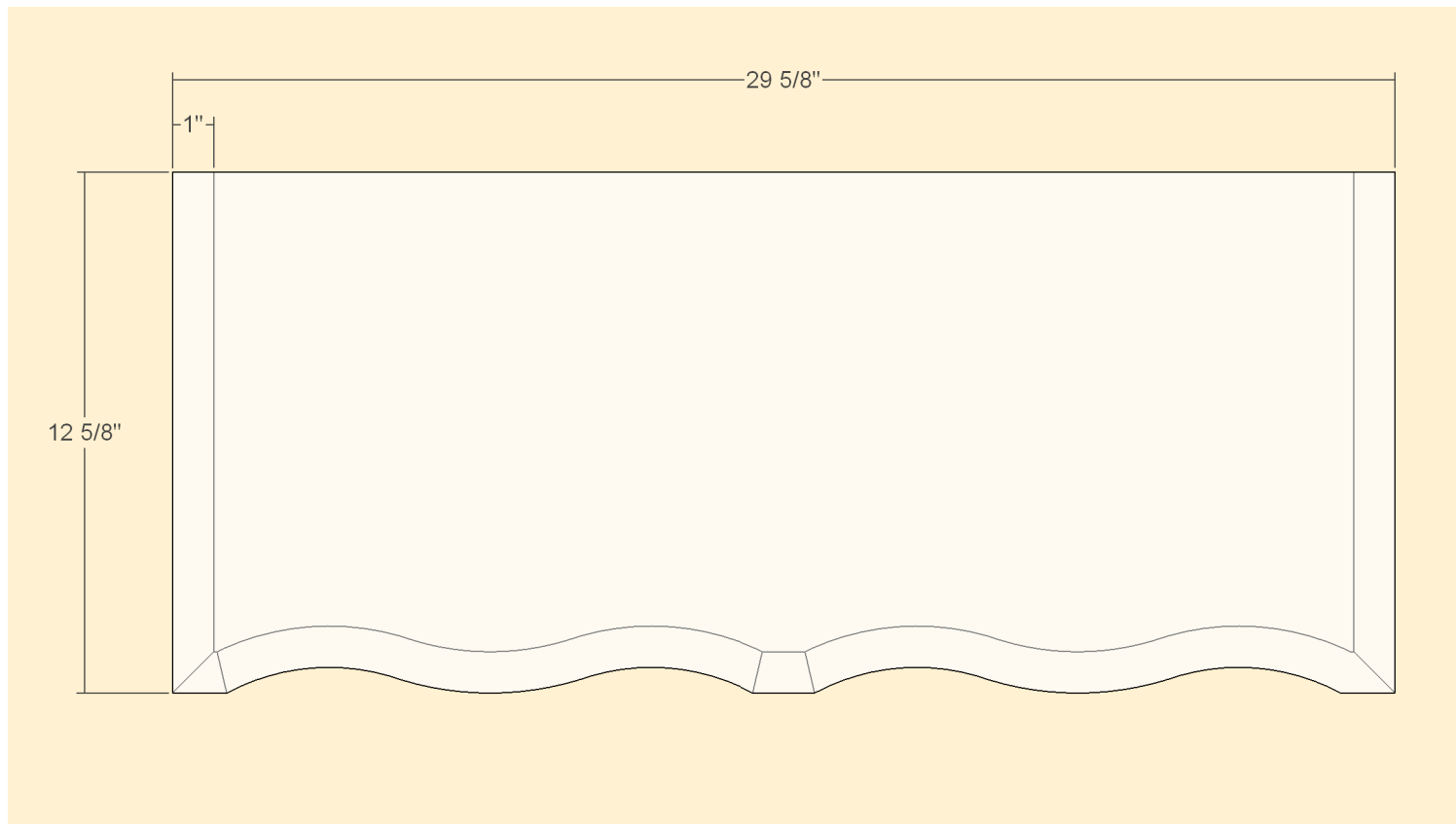
Drawer Bottom X-ray View
