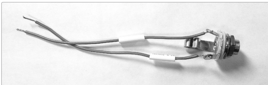
FIGURE 1-7: The prepared jack
