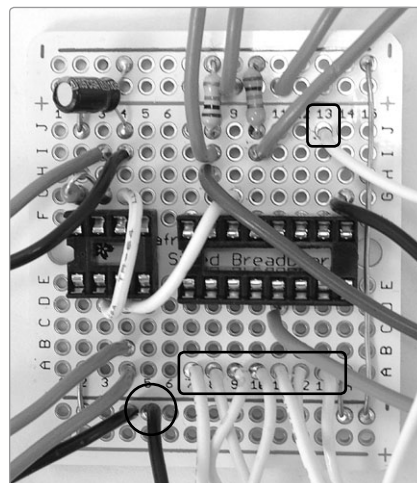
FIGURE 16-18: A wiring chart for the step controllers and a picture of the PCB thus far. The wires connecting to each step controller are white. The black-wired ground connection for the shared control LED is circled, and the step controller wires are boxed.
