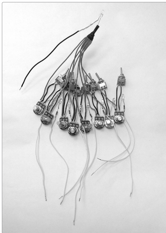
FIGURE 16-8: The finished bundle of pitch controllers connected to the control LED
