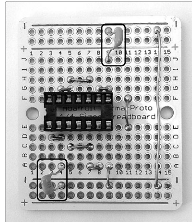
FIGURE 15-10: Mounting the 0.1 \mu\text{F} capacitors
