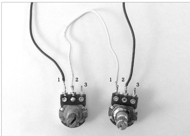
FIGURE 13-21: Daisy-chaining pots to fake your way to higher resistance
