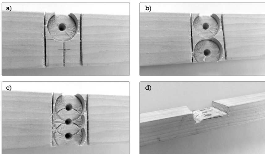
FIGURE 10-12: Routing the pickup cavity in four steps
