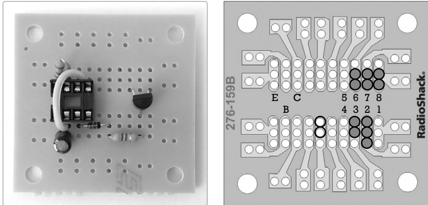
FIGURE 13-12: Placing the 470 ohm fade-in resistor
