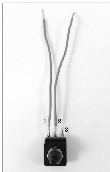
FIGURE 13-3: The prepared rate-control potentiometer
