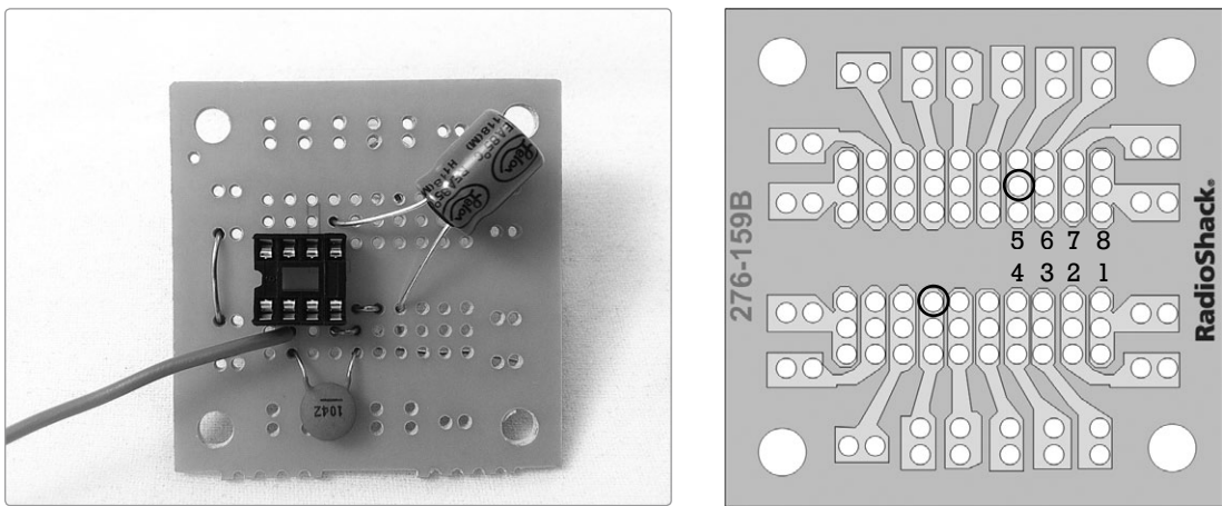
FIGURE 6-9: Placement of the 100 \mu F electrolytic capacitor
