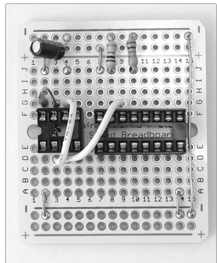
FIGURE 16-13: Adding the 1.5 \mu F electrolytic cap
