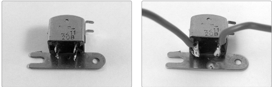
FIGURE 5-11: Wiring the four-terminal play head
