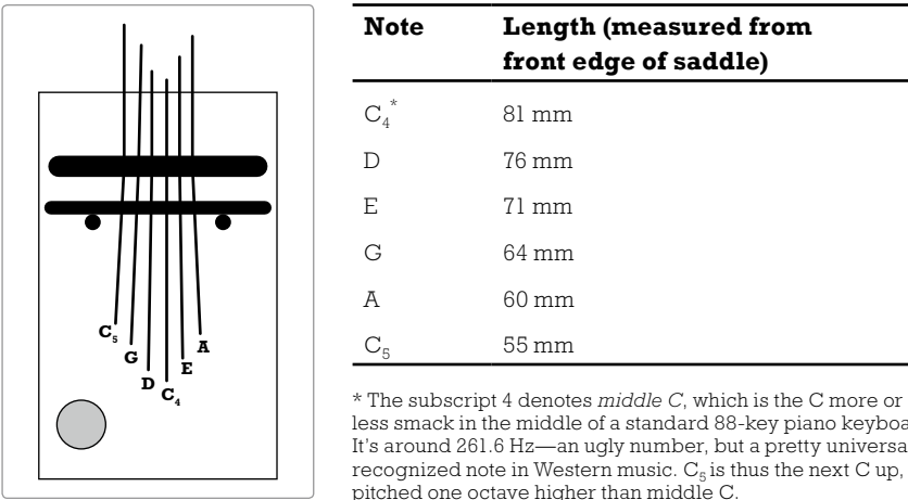
FIGURE 11-21: A diagram showing which tine corresponds to which note (left) and a chart giving the initial lengths for the six tines on your pentatonic kalimba (right)
