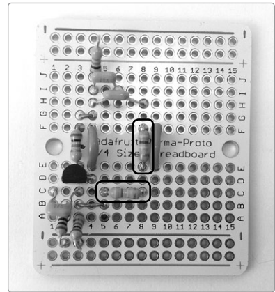
FIGURE 14-15: The two 470k ohm resistors in place
