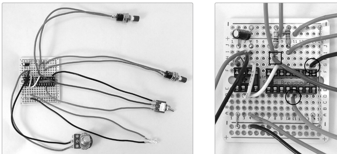
FIGURE 16-17: The rhythm selector is in place. In the detail on the right, the center-lug connection is squared and the other two lugs circled.
