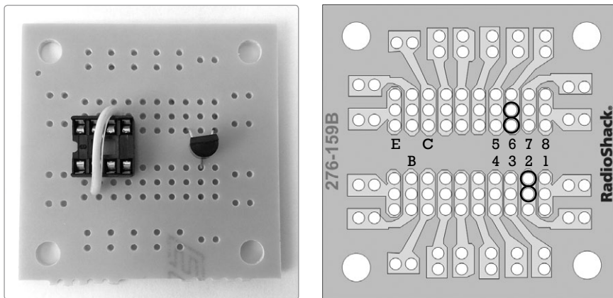
FIGURE 13-8: The placement of the first jumper (left) and the first solder points (right)
