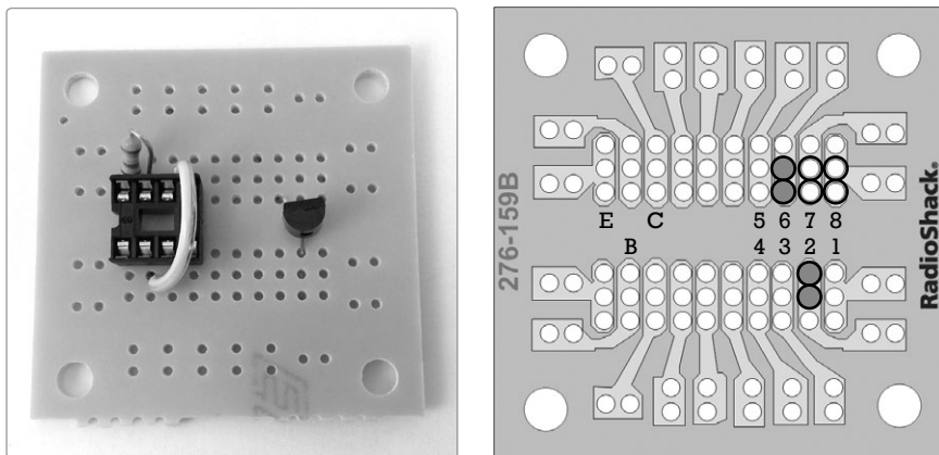
FIGURE 13-9: Placing and soldering the 120k ohm resistor. (New solder points are white; solder points from the previous steps are gray.)
