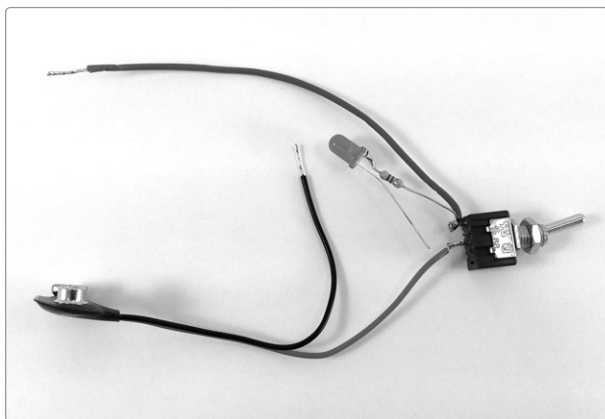
FIGURE 12-5: The completed power supply (detail of the LED assembly on the left)
