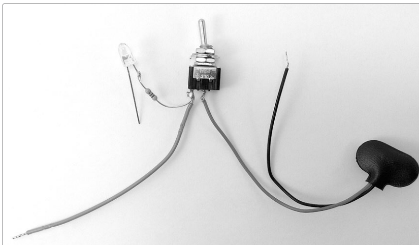
FIGURE 14-4: The finished power switch with indicator LED
