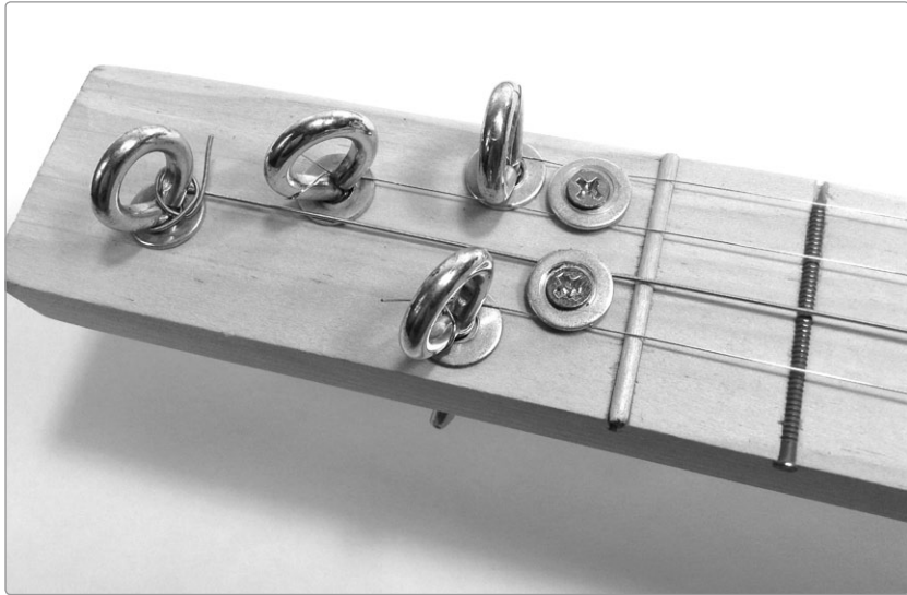
FIGURE 10-20: Placement of the string trees
