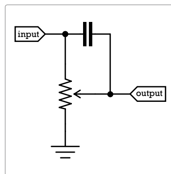
FIGURE B-11: The classic extra-presence volume control mod
