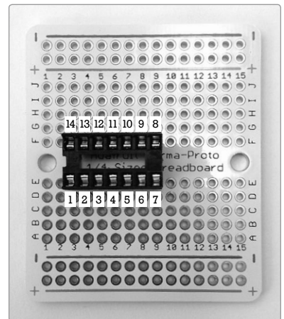
FIGURE 15-8: Positioning the IC socket. Sockets are symmetrical, but if yours has a notch at one end, as mine does, it's traditional to place that to the left so that it aligns with the orientation markings on the IC.
