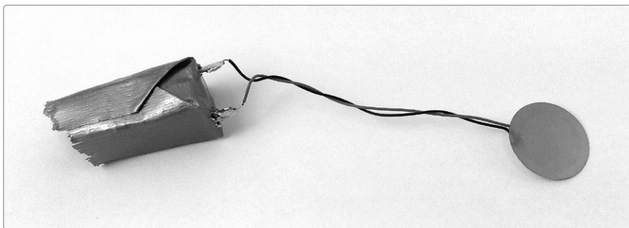
FIGURE 2-6: Twisting the two leads makes it easier to coat them in Plasti Dip.
