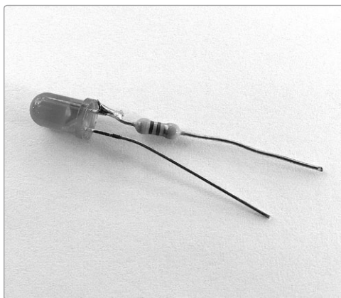
FIGURE 12-5: The completed power supply (detail of the LED assembly on the left)
