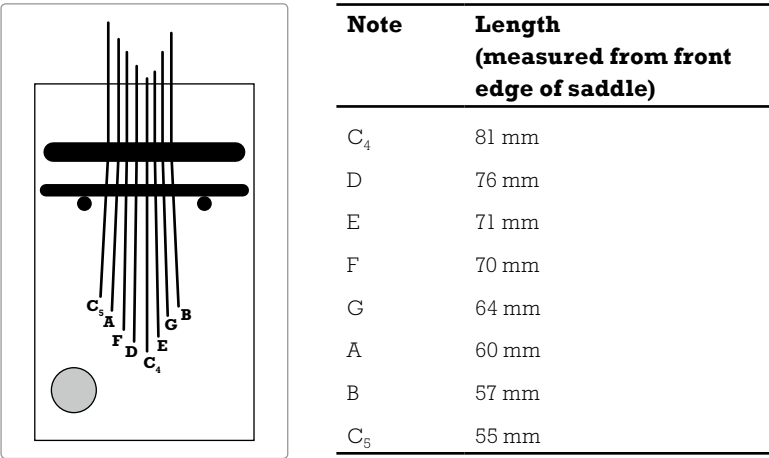
FIGURE 11-23: A diagram showing which tine corresponds to which note (left) and a chart giving the initial lengths for the eight tines on your diatonic kalimba (right)
