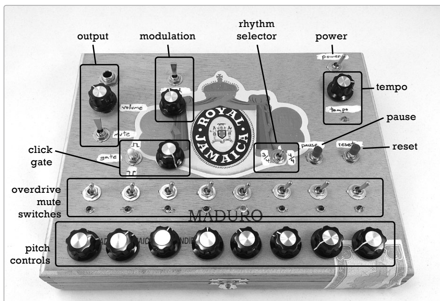
FIGURE 16-3: The Bleepbox control panel
