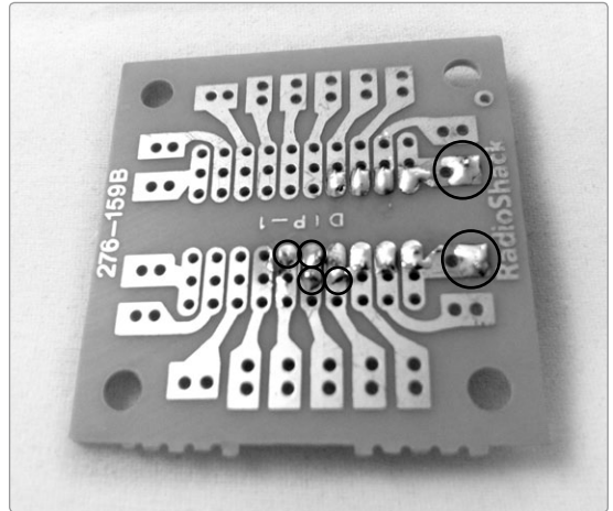
FIGURE 6-6: Running the jumpers, as seen from the top and bottom. The solder joints added in this step are circled in the right-hand image. The PCB will quickly become crowded with solder points, so we'll use a clean diagram to show the solder points henceforth.
