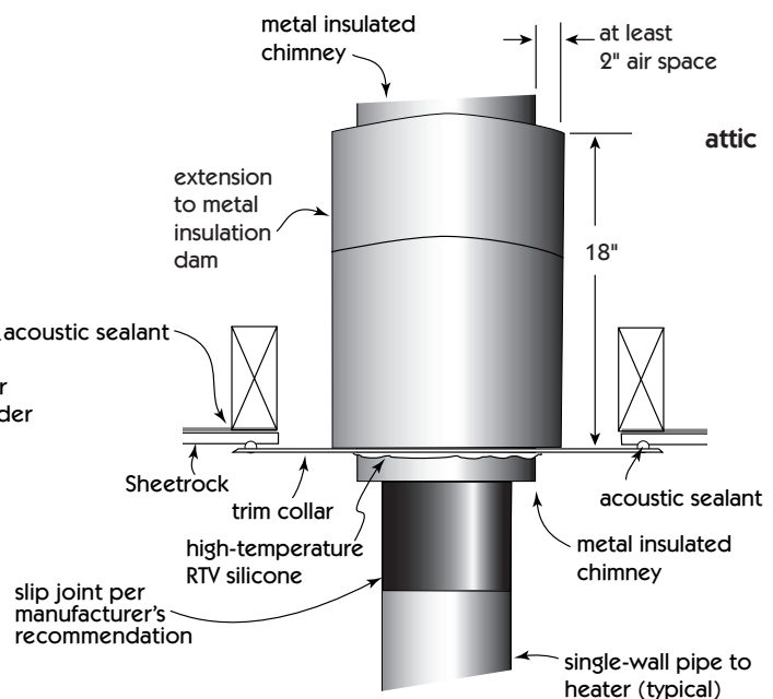
Interior side air seal (typical on retrofit)
