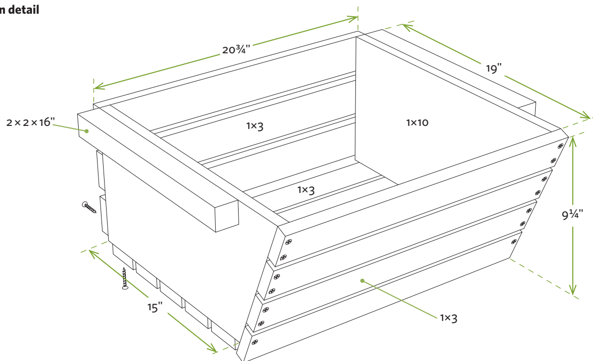
Bin detail
