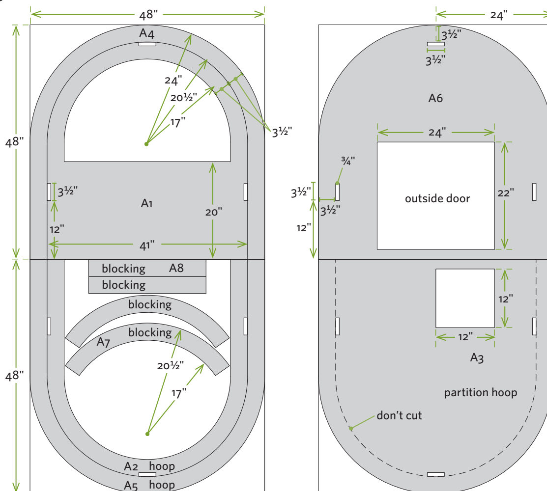
Hoop diagrams
