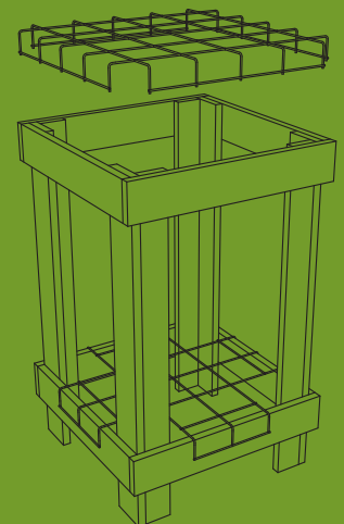
Stand-Up Tool Rack, 150
