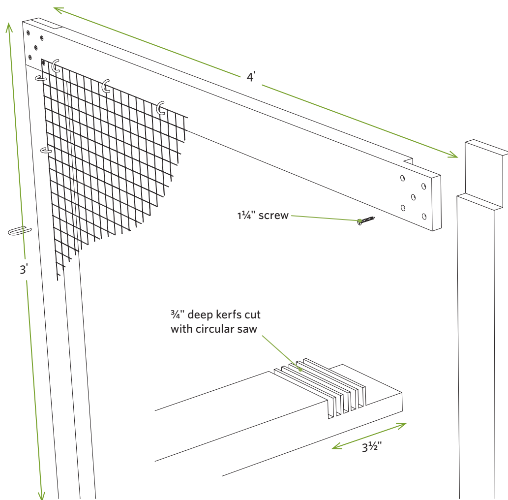
Panel construction
