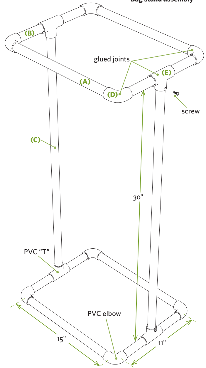
Bag stand assembly
