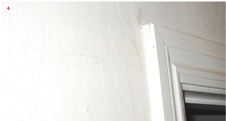
Panel joints placed too near window and door corners will tend to crack as the lumber in the header and other framing around the openings shrinks.
