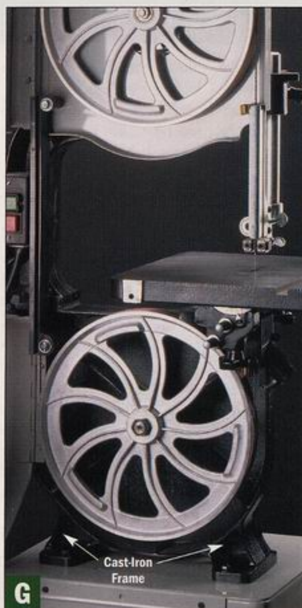
▲ Cast-iron frames have less resaw capacity out of the box, but can be expanded. The heavier nine-spoke wheels help dampen vibration.
