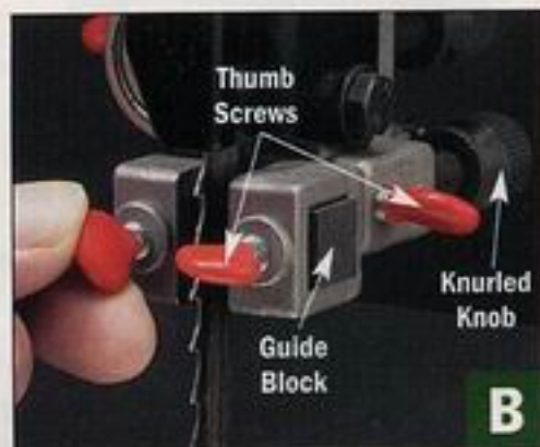
▲ Thumbscrews on Ridgid's guide system make it completely tool-less. A knurled knob positions the guides.
