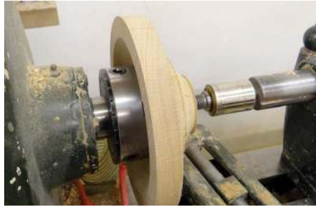
Bowl blank placed over the chuck with live centre holding it securely
