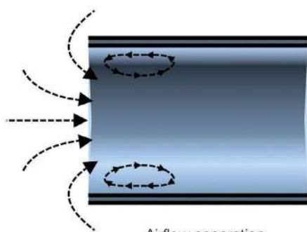
Airflow separation and recirculation at hood entrance
