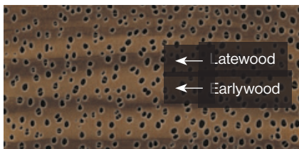
Koa (diffuse-porous) 10x scale
