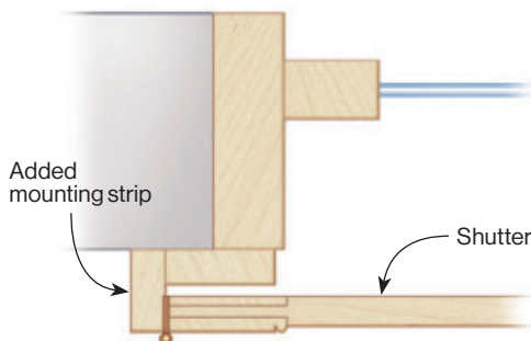
OUTSIDE MOUNT
