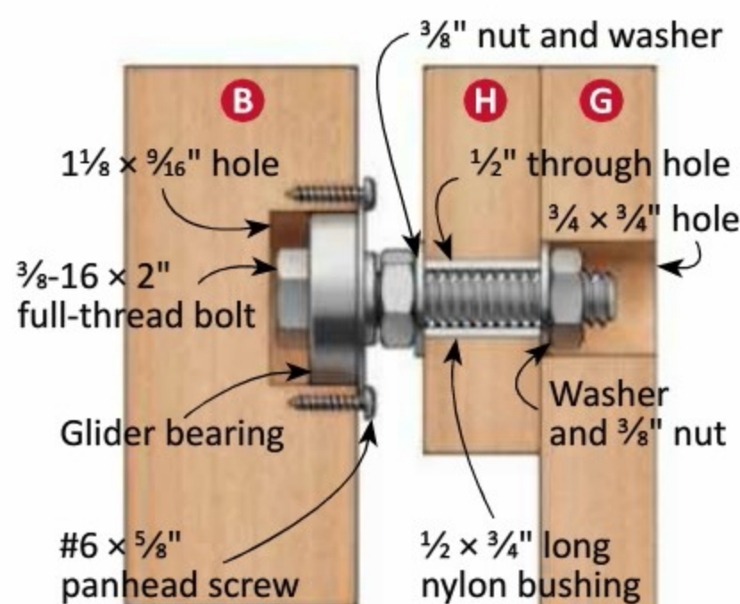
Figure 2: Glider Bearing Detail
