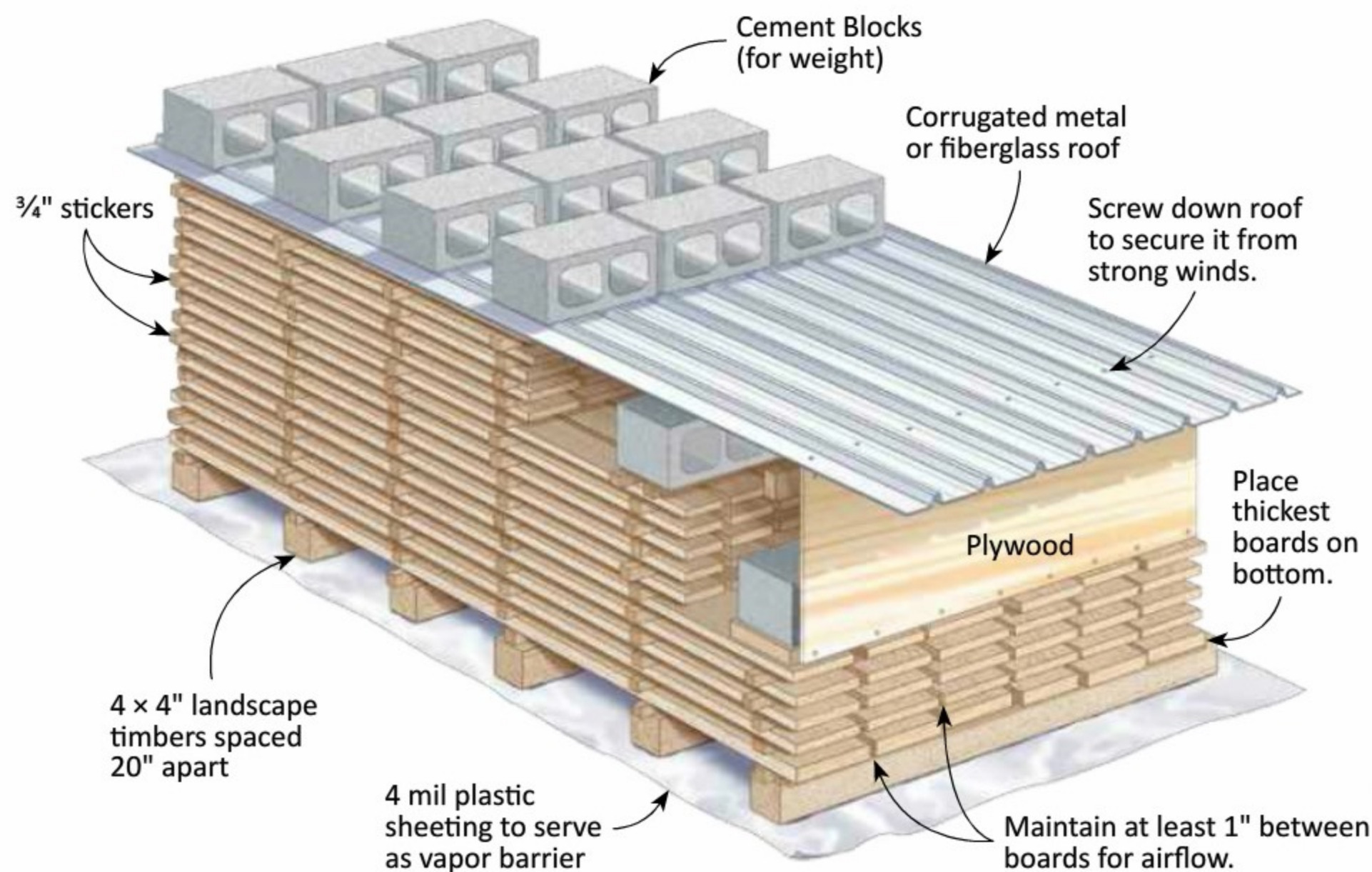
Figure 3: Building a Conventional Air-Drying Stack
