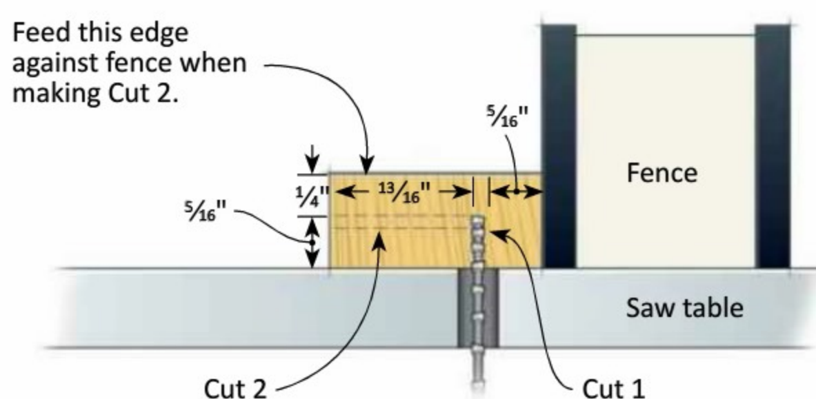
Figure 2: Base Cutting Sequence
