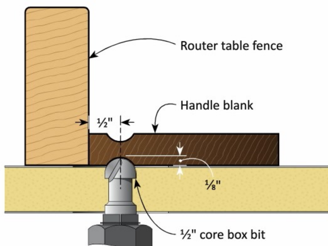
Figure 2: Cove-Cutting Setup
