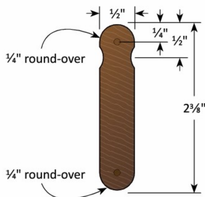
Figure 3: Handle and Brass Side Details
