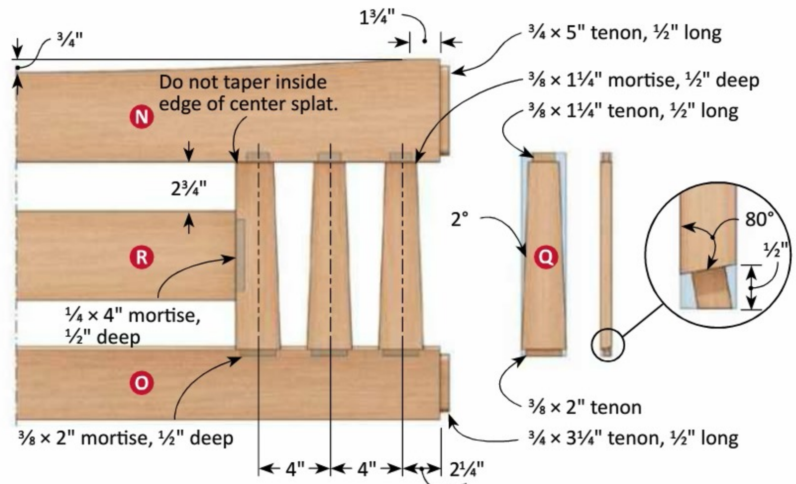
Figure 5: Back and Splat Detail
