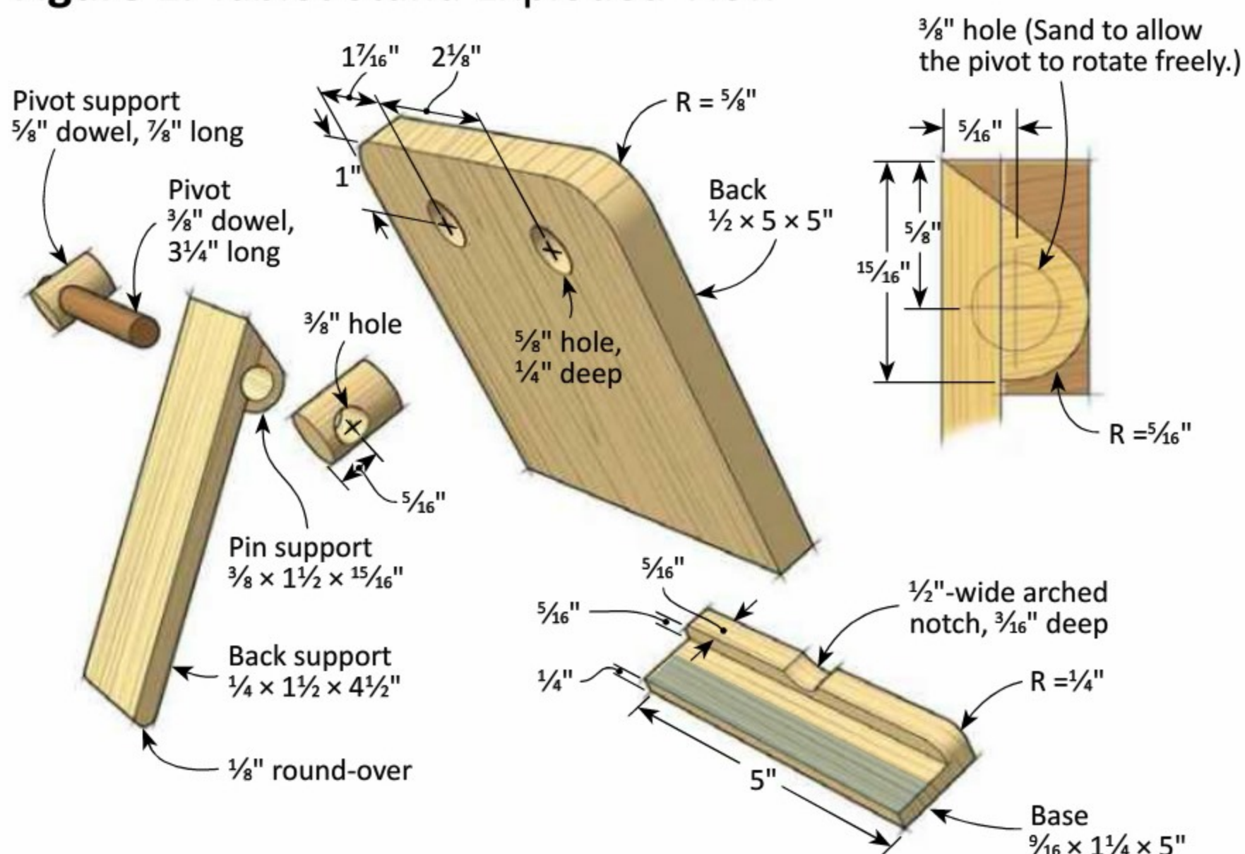
Figure 1: Tablet Stand Exploded View
