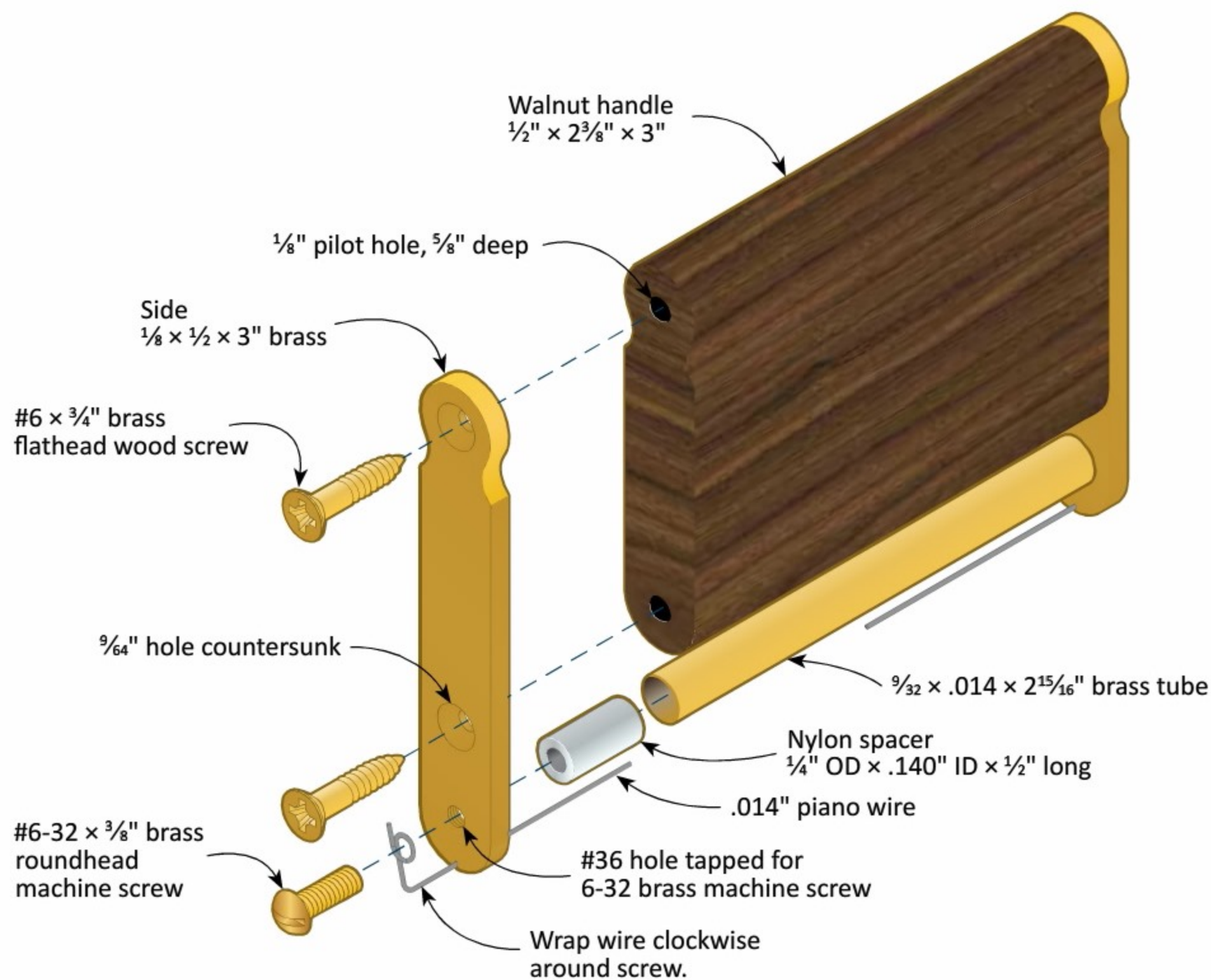
Figure 1: Cheese Cutter Exploded View
