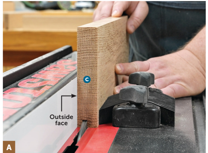
Set the blade height to \frac{3}{8} " and position the rip fence \frac{1}{4} " from the blade. With the outside face against the fence, cut an offset groove in the inside edge of each stile (A) and rail (B, C).
