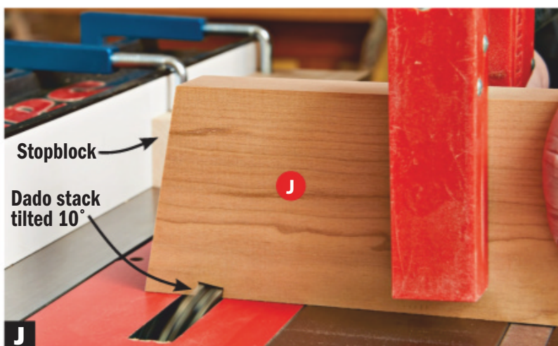
J A ½" stacked dado tilted to 10° accurately notches the backrest sides. A stopblock clamped to the fence ahead of the blade safely positions each rail for precise cutting.
