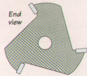
Slot-and-arbor cutter; also known as three-wing slotting cutter
