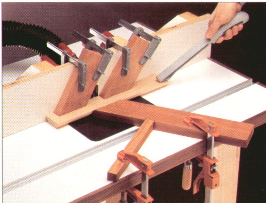
Three featherboards—two clamped to the fence and one to the table—hold the workpiece shown above safely against the fence and table while a push stick is used to feed the stock into the bit. Dust and wood chips are being extracted by a dust collection hose attached to a dust hood built into the fence.
