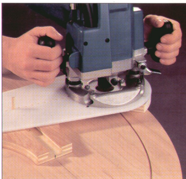
Paired with a commercial circle-cutting guide, an oval-cutting jig guides a router as it plows an elliptical groove for decorative inlay banding in a tabletop. The jig was used in a series of successively deeper passes to rout the table's outline. Refer to page 84 for instructions on making this easily adjustable jig.
