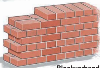
Blockverband
