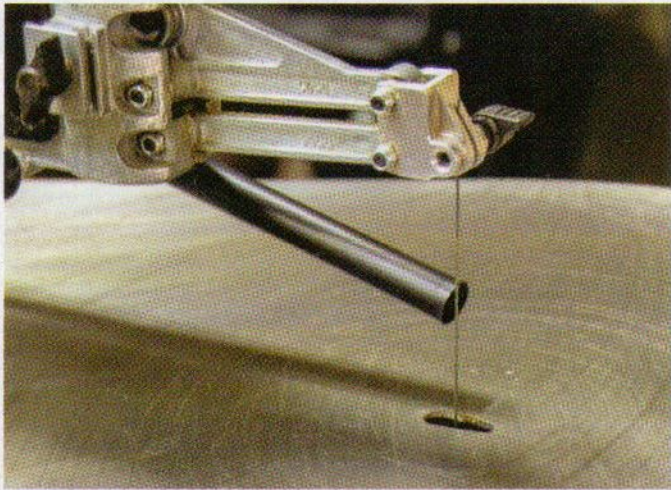
The upper collection hose captures dust from the top of the project, instead of blowing it away.
