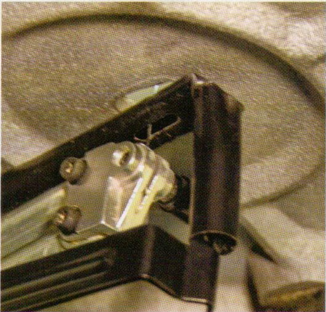
The lower collection hose mounts directly below the cutting area, and the blade actually passes through it.
