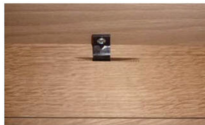
Metal or buttons. You can use metal connectors as I did, or wooden buttons to connect the top to the carcass. Either way, offset the slots in the case sides by \frac{1}{16} "- \frac{1}{8} " so the top pulls down tight.
