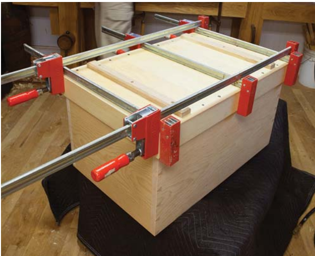
Yes, clamp. Glue the short grain of each miter and clamp it at the corners. The glue will have more strength this way.
