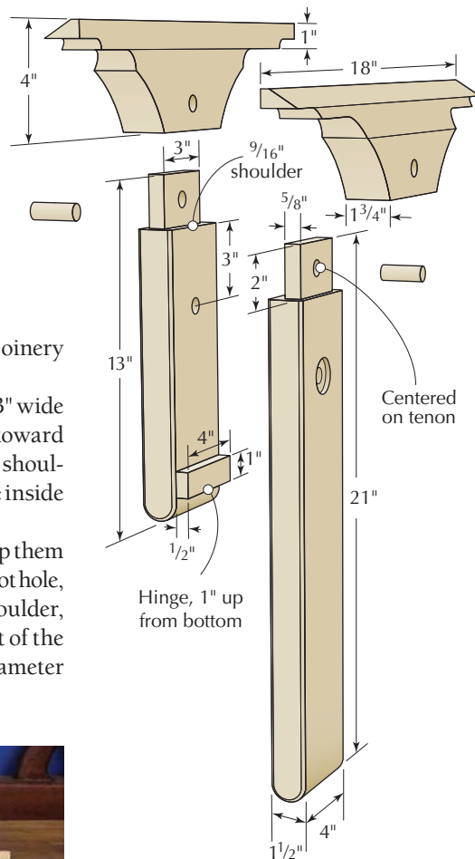
EXPLODED VIEW
