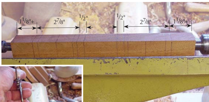
One blank; two balusters. This 1" x 1" x 10" blank will yield two balusters.
