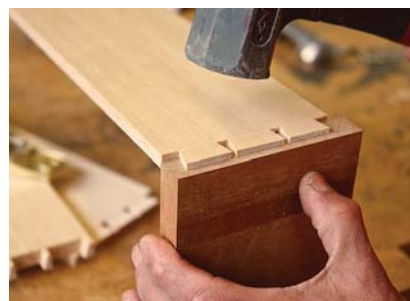
Half-blind. At the front, the drawers are joined with half-blind dovetails (through-dovetails are used at the back).
