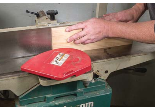
Kumiko stock prep. Start with finish-planed \frac{3}{4} "-thick boards. Joint both edges flat (left), then finish plane (center) before band-sawing strips a bit thick (right). This leaves just one surface to finish-plane after the pieces are cut.
