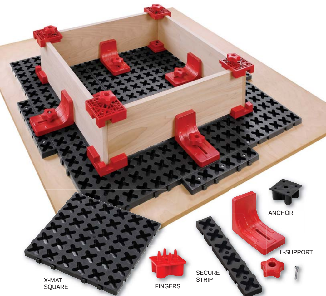
X-Mat L-Supports
