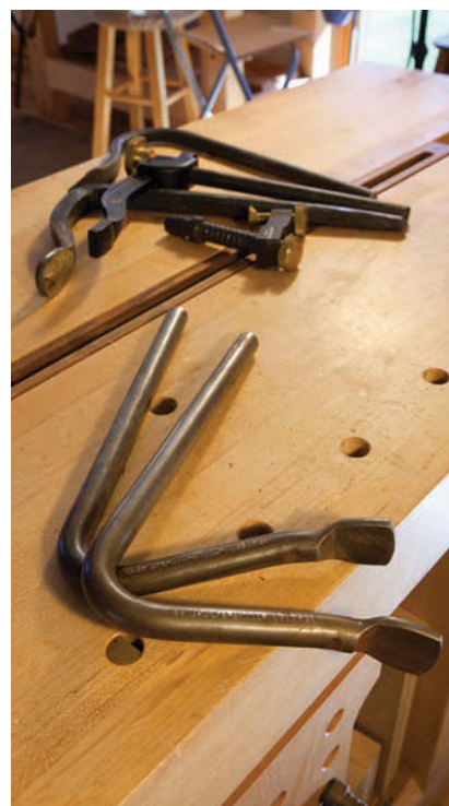
Gramercy Holdfast. This wire-formed holdfast (foreground) is the least-expensive effective holdfast on the market.
