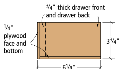
Drawer detail
