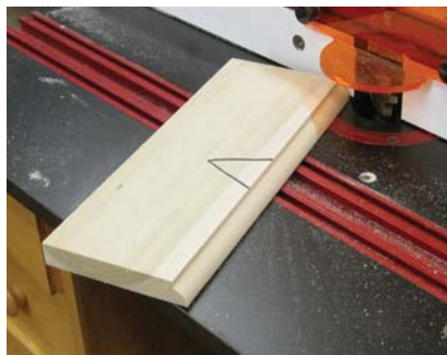
Router it out. Riding against the length of the fence rather than off a bearing does a better job of routing a straight profile on the leaves.
