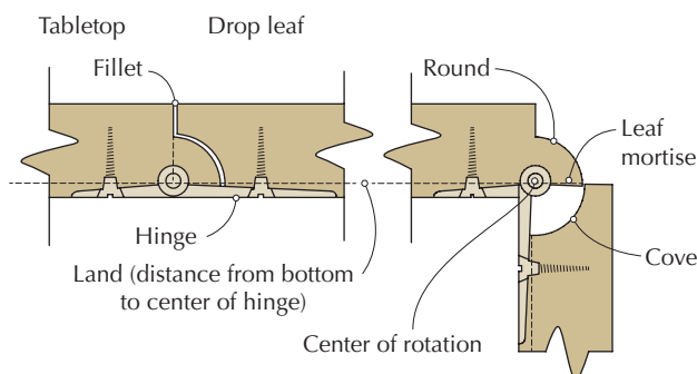
HOW A DROP LEAF WORKS
