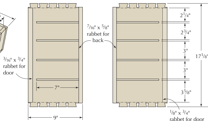
SIDE LAYOUT
