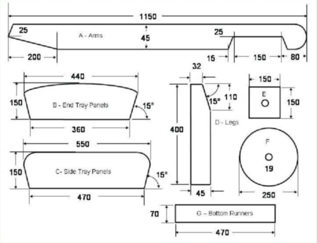
Fig. 2: Shaping of parts
