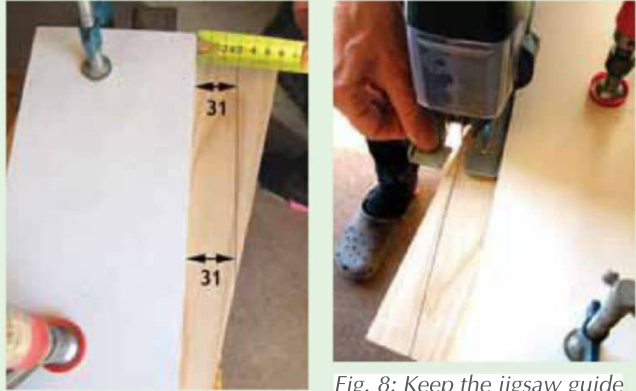
Fig. 7: Clamp a piece of scrap wood to the workpiece
