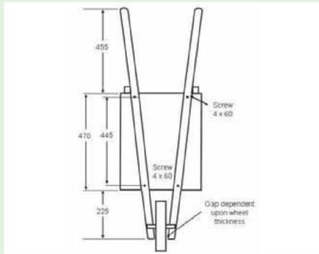
Fig. 17: Attaching the arms to the tray
