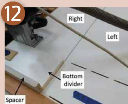
Biscuiting setup #2
