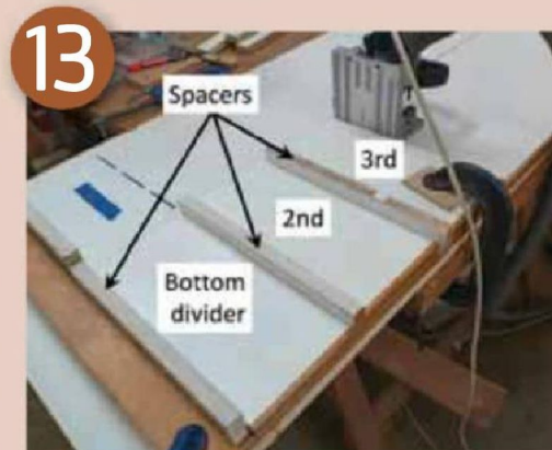
Biscuiting setup #3
