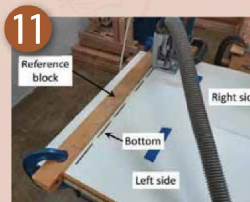
Biscuiting setup #1
