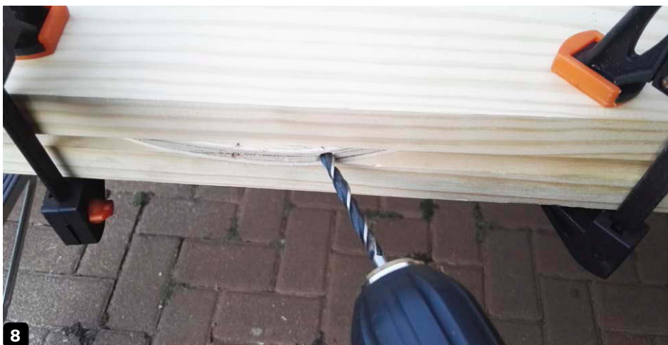
With the board clamped safely in place drill holes for the dowel sticks
