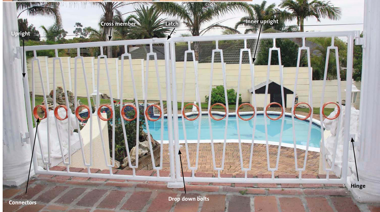
Diagram of the gate components
