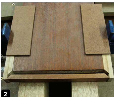
2 Mitred edging applied to veneered material
