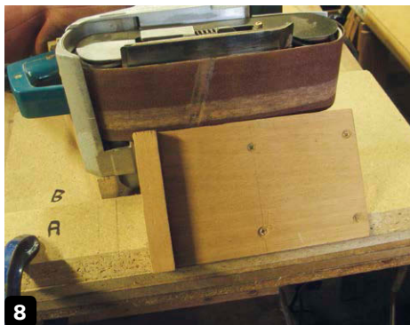
8 Set-up to sand mitres
