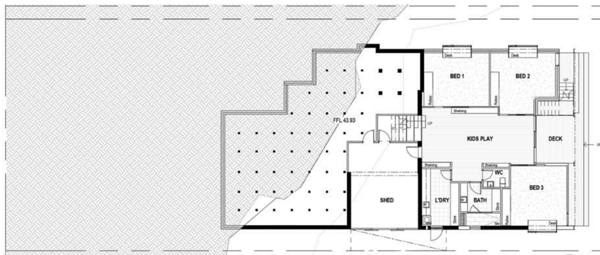
Lower Ground Floor Plan
