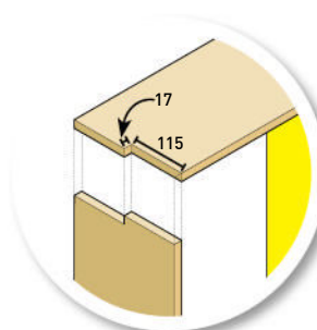
JOINT DETAIL
