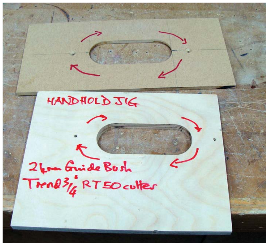
Master and production jigs cut and labelled
