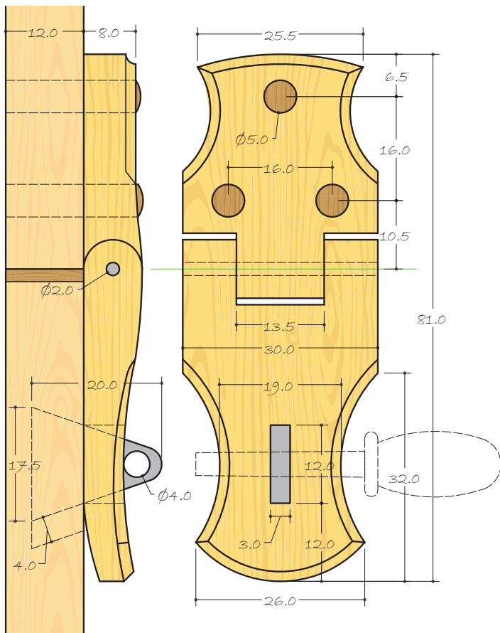
FRONT & SIDE ELEVATIONS OF CLASP Scale 1 to 1
