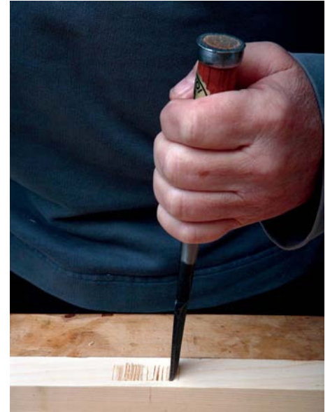
Chopping a mortise, starting from the centre moving outwards, the oire nomi chisel's bevel is angled away from the centre
