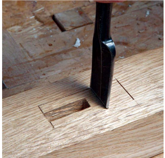
The broad shallow outer mortise is chopped on the entry face
