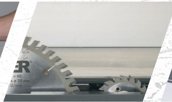
Scoring unit Tear free cut for laminated workpieces
