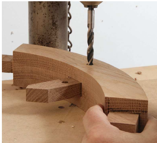
Drill through the mortised parts. Insert a scrap into the mortise to prevent blowout inside.
