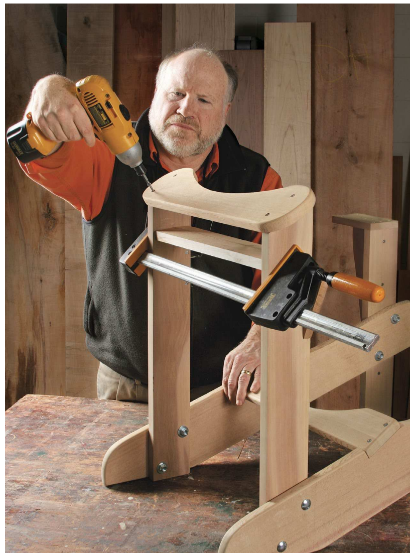
Attach the upper cradle. Use a temporary spacer board to ensure that the risers stay parallel when the upper cradle is attached.
