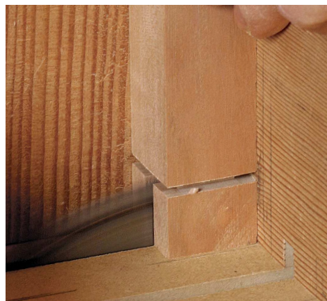
Begin in the middle on the double tenons. Once you've cut the shoulders, cut away the waste between the tenons in the middle of the stock (left). Cut the inside face of one tenon, then rotate the stock 180° for the second cut. Creep up on the right distance, using the leg to check the fit. Finally, cut the outside cheeks and ends (right).
