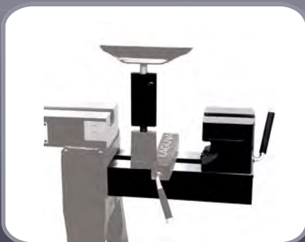
20" EXTENSION W TAIL-STOCK BASE & TOOL-REST EXTENSION
