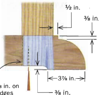
SHOE DETAIL
