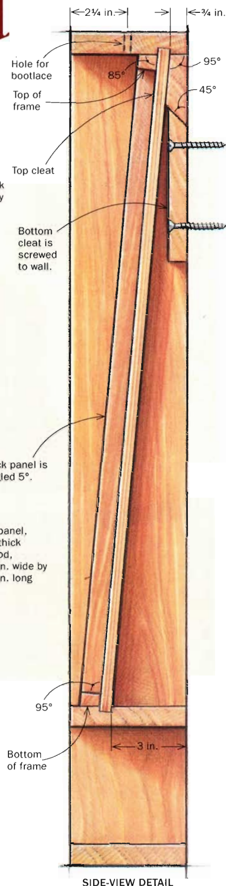
SIDE-VIEW DETAIL
