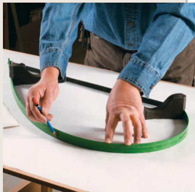
Heavy helping hands. It's tough to hold the bow and trace a line at the same time. If you don't have a helper, use spline weights, often called whales by boatbuilders, to keep the bow still as you scribe the curve.
