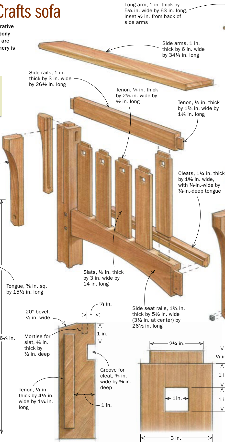
SEAT-RAIL DETAIL
