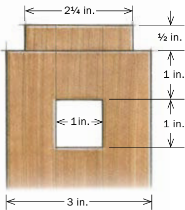
SLAT DETAIL
