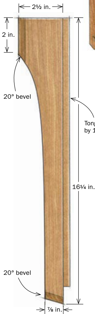
CORBEL DETAIL
