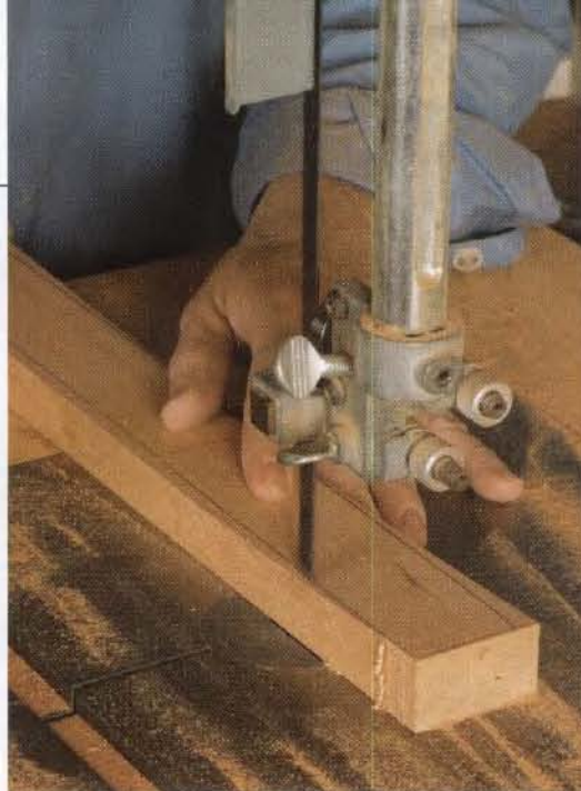
Bandsaw curves. Begin with the curve for the top of the armrests (above), then bandsaw the curves for the sides (right).
