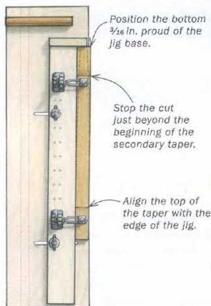
Set up a stopped cut. Clamp a hook-shaped stop to the fence so that you don't completely remove the waste from the long-taper cuts.
