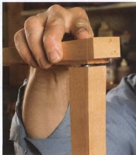
Drill for dowels. Use \frac{3}{8} -in.-dia. dowels to connect the legs to the armrests. Drill the legs first, then use dowel centers (left) to locate the holes in the armrests. Position the armrest and press down (right). Now you can drill the mating hole in the armrest.
