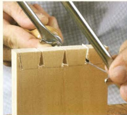
A coping saw cuts out the waste. Setting the blade at a 45° angle makes it easier to turn the sharp corner at the bottom of the backsaw cut and cut the waste away. Leave about 1/16 in. of material above the baseline. Pare it away with a narrow chisel to complete the process.
