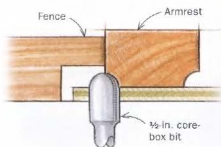
Route a cove on the underside. The cove gives the thick armrest a lighter look. Edmundson uses a narrow shopmade guide that clamps to the router table and sits above the blade. It follows both the convex and concave sides of the armrests. Reset the stop for the end-grain cuts.
