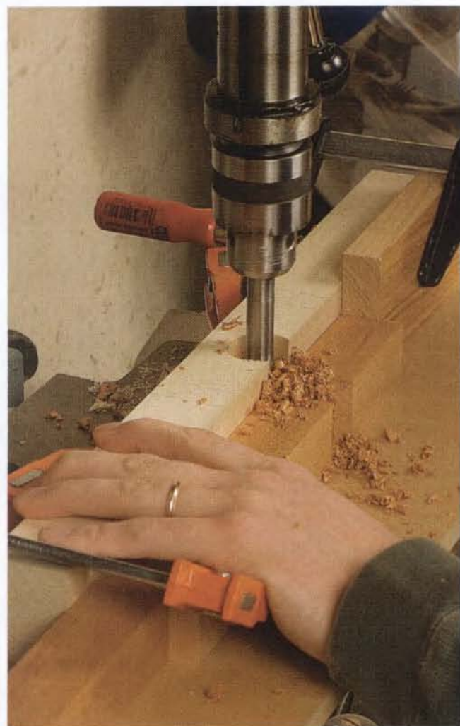
Drill hollows in the leg. Clamp a leg blank against the hardwood fence, aligning the ankle with the drilled-away edge of the fence. Drill a hollow in each side of the blank.
