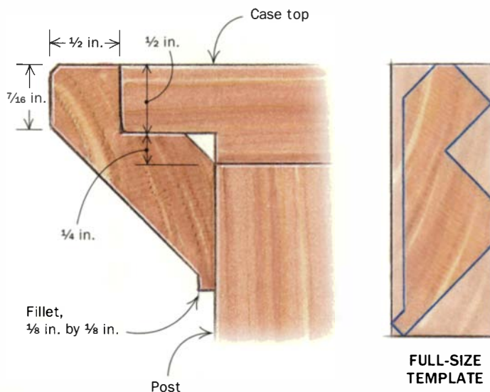
Tack the cornice into place. The molding's angular profile accentuates the square corners of the piece.
