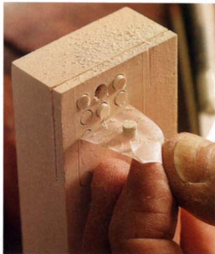
Custom plug cutter. The author files teeth on the end of a brass rod (above) and uses a drill press to drill the holly plugs. Clear tape prevents the plugs from falling out when slicing them free with a handsaw (right).
