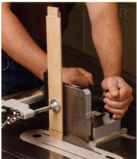
Rail tenons look lopsided. The joinery needs shoulders of different heights to seat properly in the rabbeted stiles.
