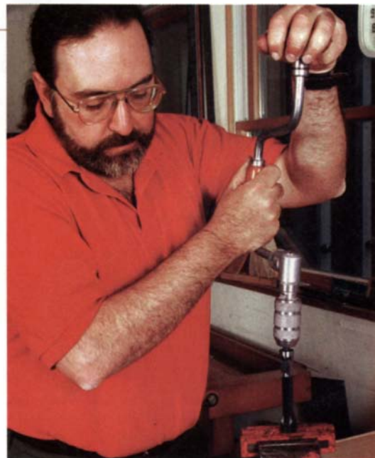
Interchangeable pilots. The reamer comes with an assortment of pilots to fit various sizes of chisels.
