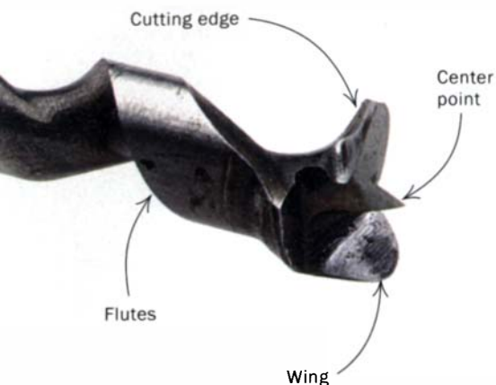
Start with the wing. A few short strokes with a fine-grit auger-bit stone sharpens the wing of the bit.
