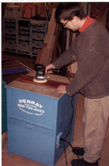
Attacking dust at its source. Denray's compact, industrial-quality downdraft table draws air through its filter at the rate of 1,500 cubic feet per minute.
