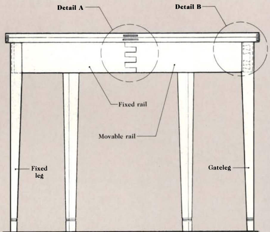
Back View
