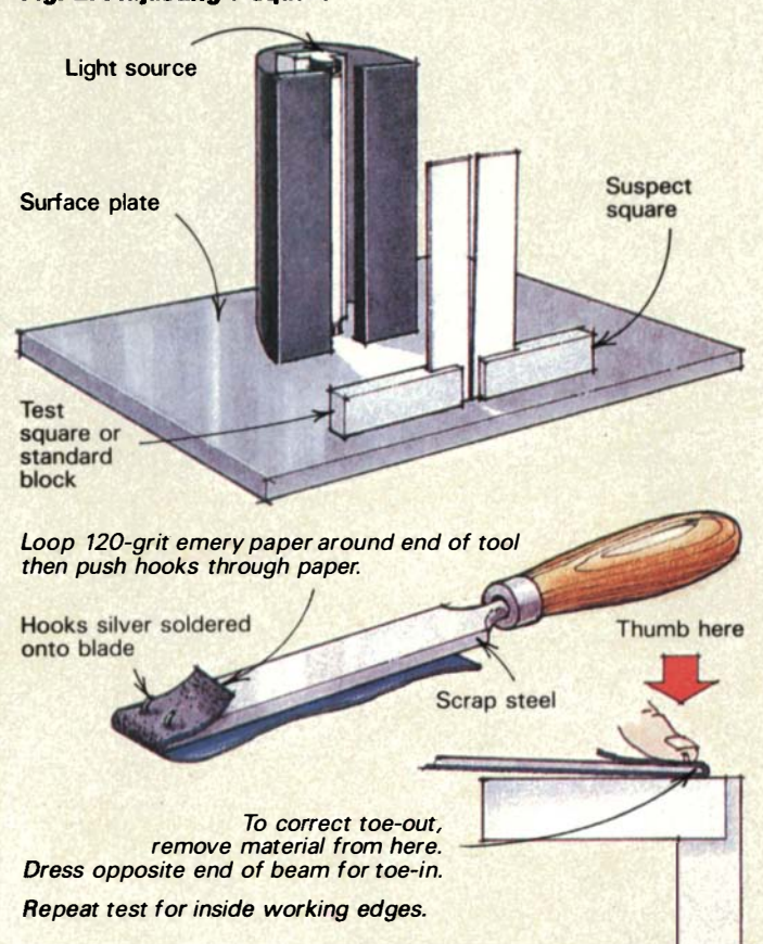
Fig. 2: Adjusting a square
