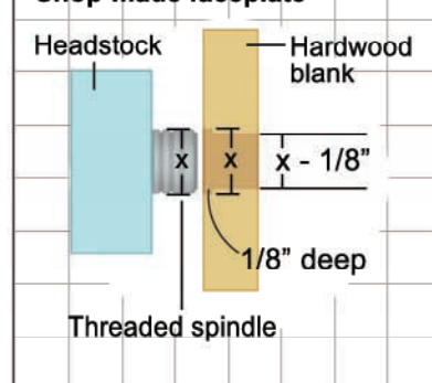
Shop-made faceplate
