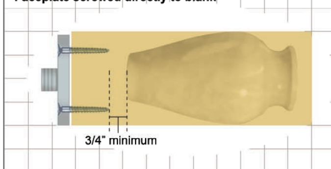
Faceplate screwed directly to blank
