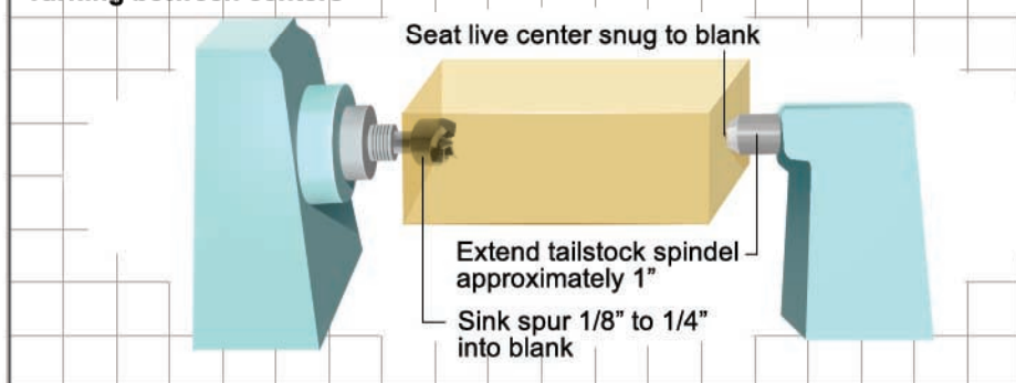
Turning between centers
