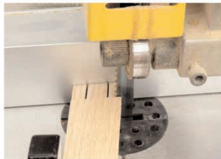
Cut square tenons on band saw
