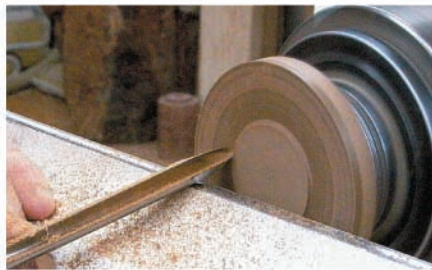
Make a facing cut across the face
