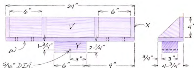
Fig. E Caster Brackets
