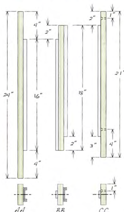
Fig. H Slide Support Dimensions
