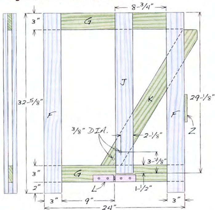
Fig. B Cabinet Frame Dimensions
