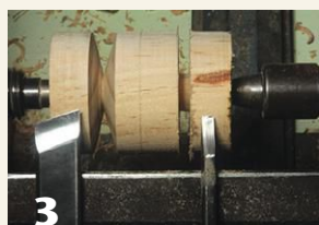
Shown at left is a symmetrical V-groove made with a skew's long point; at right, a rectangular trench cut with a parting tool.
