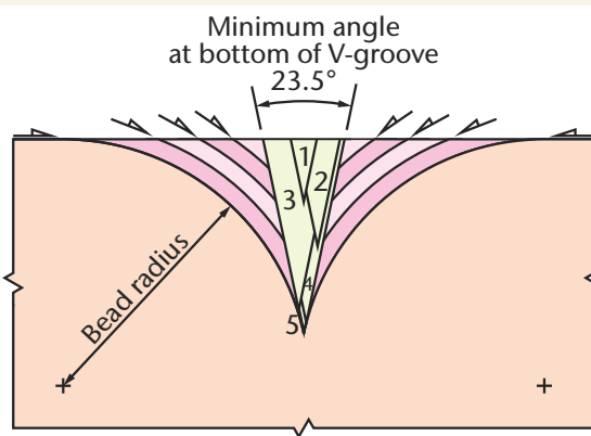
Figure 2. The cut sequence for a symmetrical V-groove. If using a symmetrical V-groove alongside an isolated bead, it's better to make the last cut of the series on the bead side of the V-groove. The arrows represent the tilts of the skew's short point at the start of each rolling cut.
