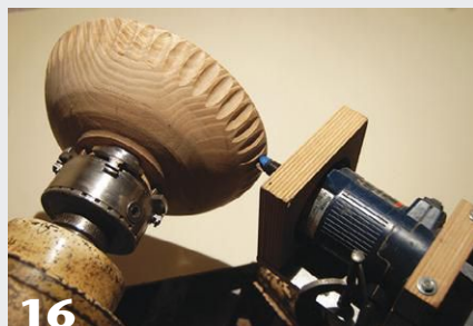
16 With the router mounted perpendicular to the turning axis, many possibilities exist for rim treatments.
