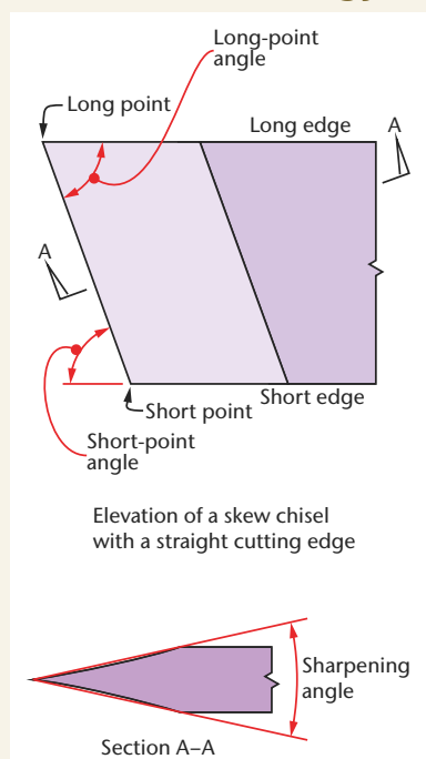
Figure 1. Terms associated with the nose geometry of a skew chisel. The long-point angle need not equal the short-point angle.
