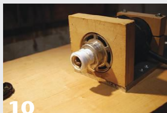
10 Router mounted in carriage with PVC depth gauge collar.
