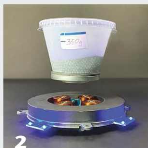
(1) The Lusya load-bearing magnetic levitation module.
