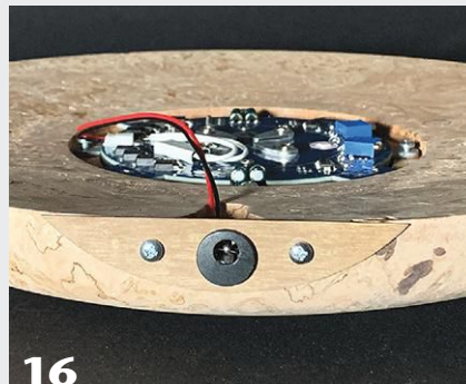
Carve a channel on the bottom of the base to accommodate the adaptor plug and wires. Test-fit the electromagnet and adaptor plug before applying a finish.
