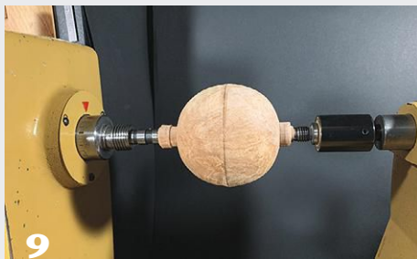
9 Turn the sphere, being sure to stick to the predetermined diameter (in this case, 4\frac{1}{2} "). The glue line is nearly imperceptible.
