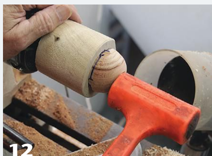
12 Before hollowing the second half, give the sphere a tap with a dead-blow hammer to ensure a snug fit. Then hollow the second half as you did the first half.
