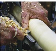
Myron's favorite tool was a roundnose, or drop-nose, scraper.
