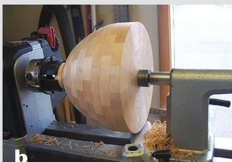
A traditional ring-segmented bowl is turned, with an extra ring pressed (but not glued) to the rim with the tailstock. After it is turned flush, the extra ring is removed and cut into the shape of a basket handle.
