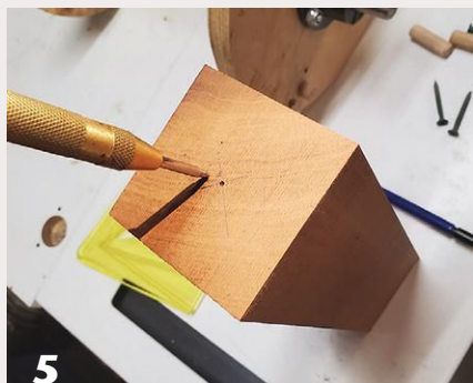
5 Mark the center at the ends of the spindles, and drill ½"-diameter holes to accept the pivot dowels.
