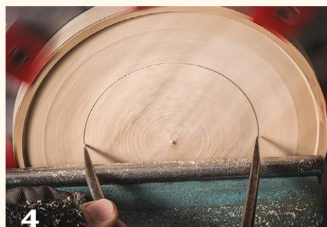
Making a 7½"-diameter plate, the author chooses his largest chuck jaws for remounting the work. Using dividers, he marks the necessary spigot, or tenon, size on the bottom of the plate.
