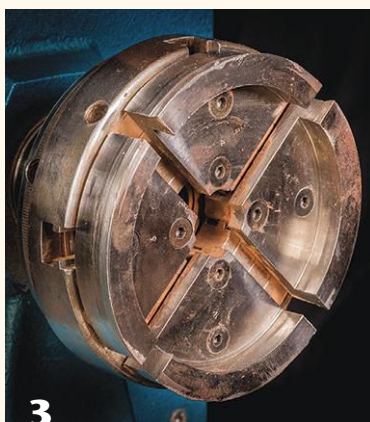
Making a 7½"-diameter plate, the author chooses his largest chuck jaws for remounting the work. Using dividers, he marks the necessary spigot, or tenon, size on the bottom of the plate.
