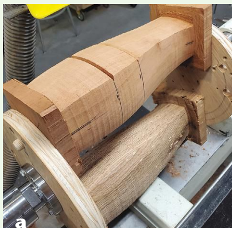
a Several of these vases were turned two at a time on the thermoing rig.
