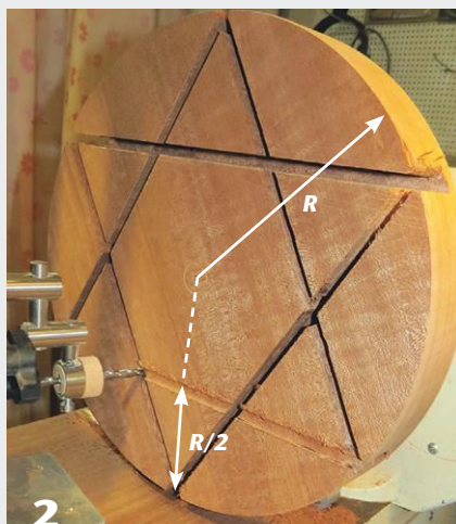
2 The depth of cut is controlled by an adjustable wooden ring on the cutter, whose height is equal to half the radius of the workpiece.
