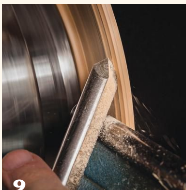
9 A small chamfer cut on the underside of the rim allows for easy gripping of the plate when in use.
